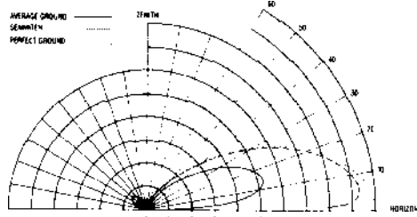
ELEVATION PATTERN (VOLTAGE) AT 3 MHz CURVES FOR VARIOUS TYPES OF GROUND
