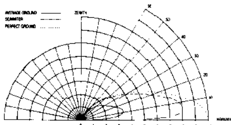
ELEVATION PATTERN (VOLTAGE) AT 30 MHz CURVES FOR VARIOUS TYPES OF GROUND
