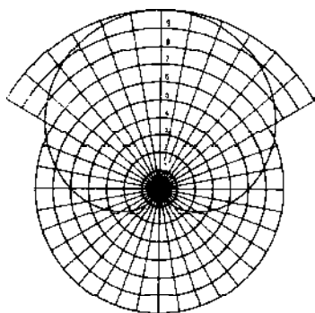
AZIMUTH PATTERN (VOLTAGE) FREQUENCY - 8 MHz
