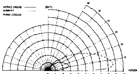
ELEVATION PATTERN (VOLTAGE) AT 12 MHz CURVES FOR VARIOUS TYPES OF GROUND
